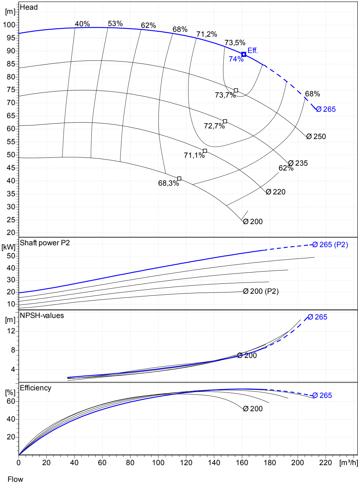
NPSH-value without safety margins
