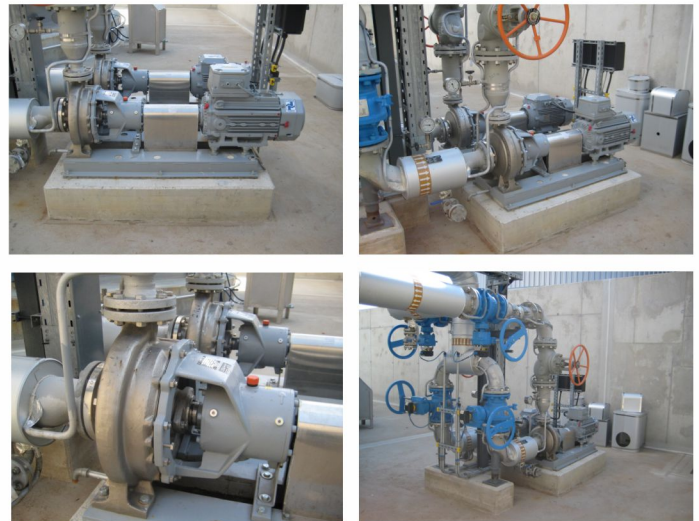
Centrifugal pump on working and pumping tanks for moving crude oil.
